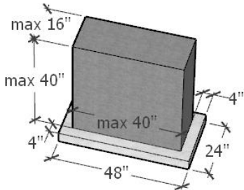
Upright or Flat Marker in Blocks 1,3,6,7,11
